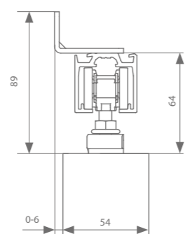
fixation murale 54 mm
