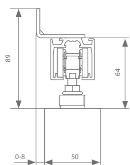
fixation murale 50 mm
